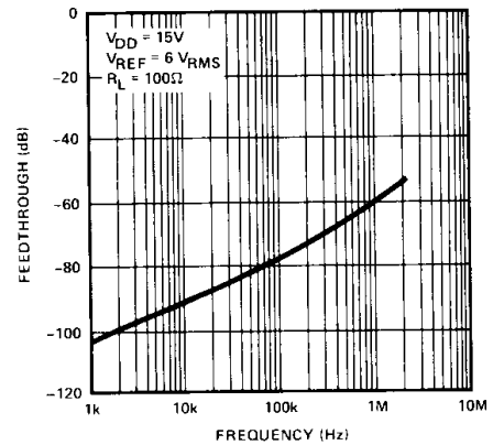
FEEDTHROUGH vs FREQUENCY
