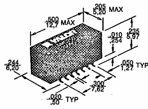
14 PIN STD SOIC Gull Wing Configuration
