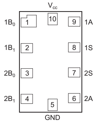
Figure 4. 10-Lead Micropak
