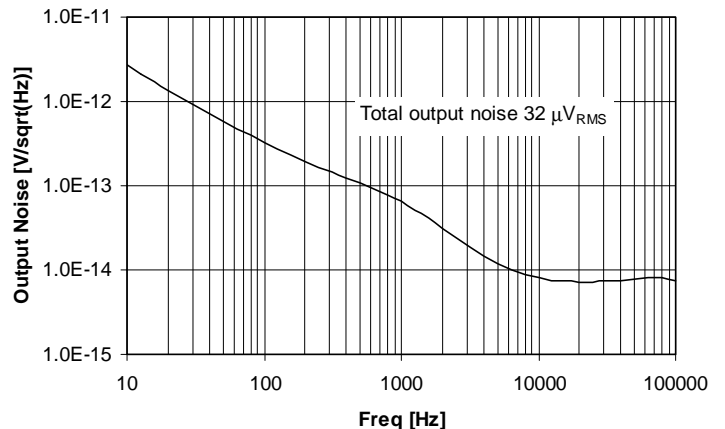
Output Noise Spectrum at Full Load for TRIMLDO3 = 0, V BAT = 4.25V and C L = 2.2 μF
