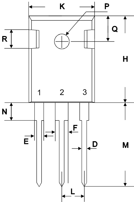
TO-247AC
