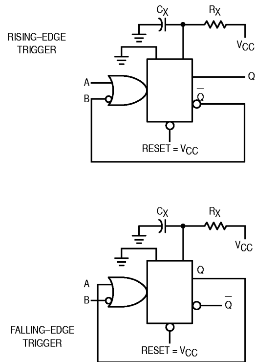
Figure 13. Non-retriggerable Monostable Circuitry
