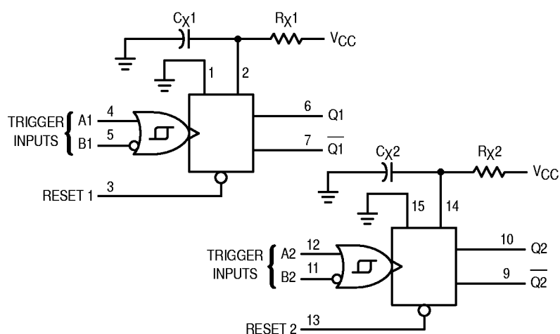
LOGIC DIAGRAM
