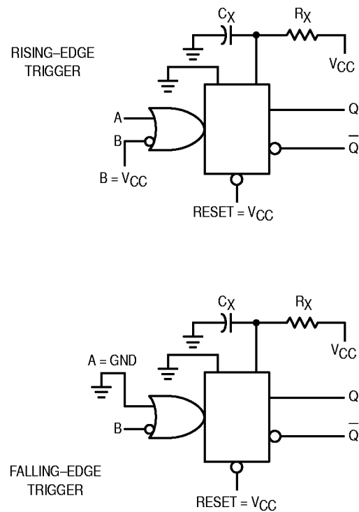
Figure 12. Retriggerable Monostable Circuitry
