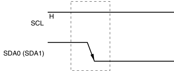
Figure 17-15. Start Condition
