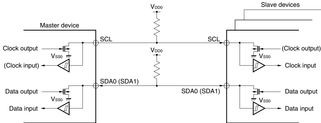
Figure 17-21. Pin Configuration
