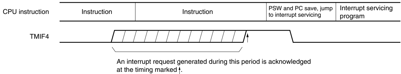
Figure 21-11. Non-Maskable Interrupt Request Acknowledgment Timing
