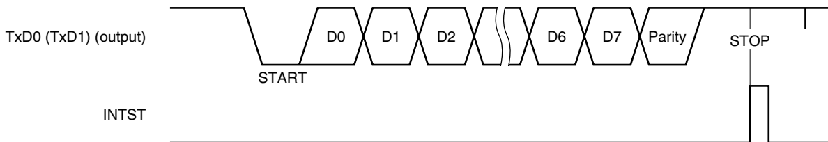
(b) Stop bit length: 2
