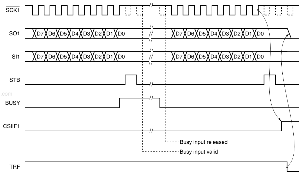
Figure 18-21. Operation Timing When Busy &amp; Strobe Control Options Are Used (When BUSY0 = 0)
