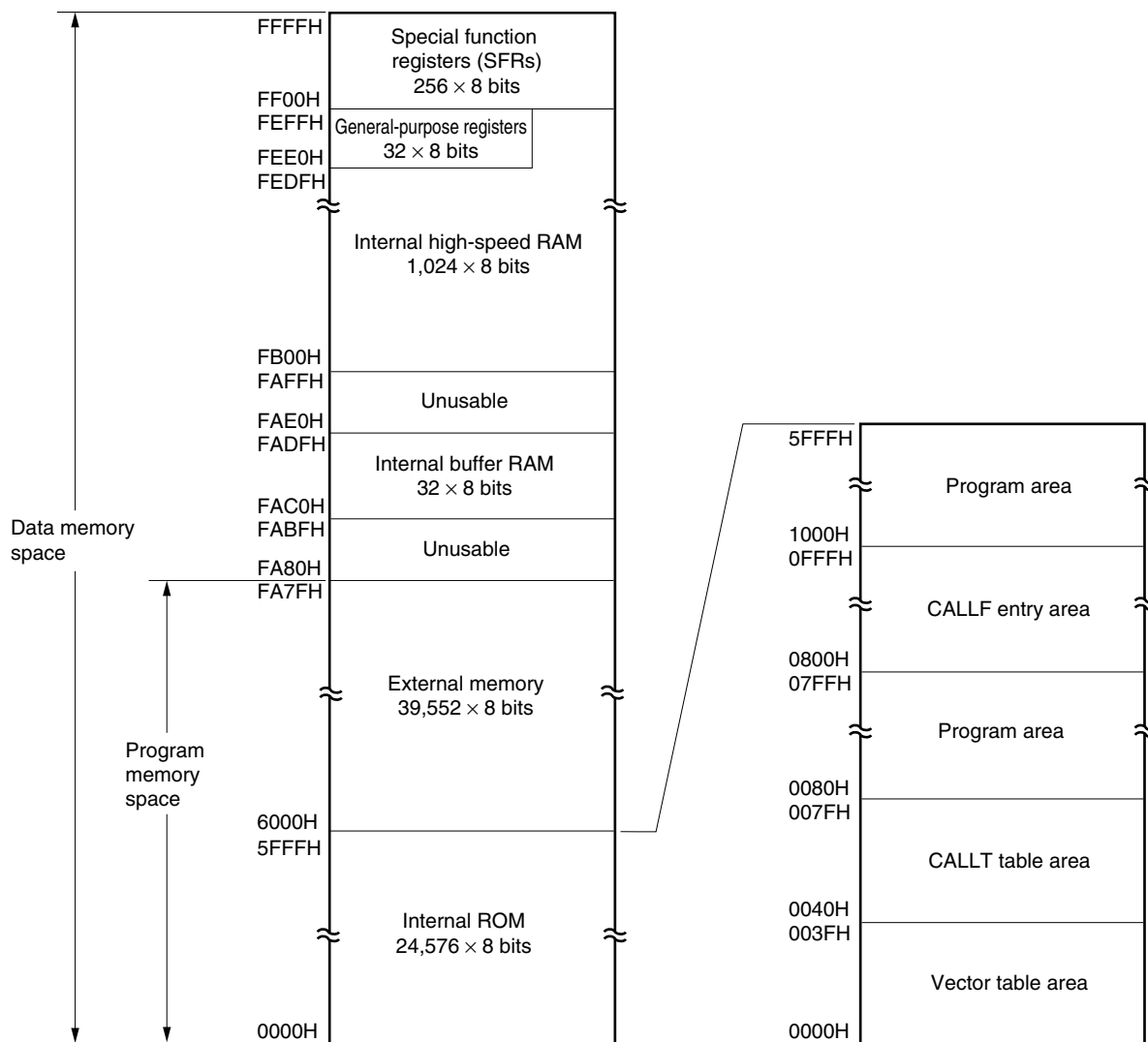
Figure 5-1. Memory Map ( \mu PD780053, 780053(A), 780053Y, 780053Y(A))
