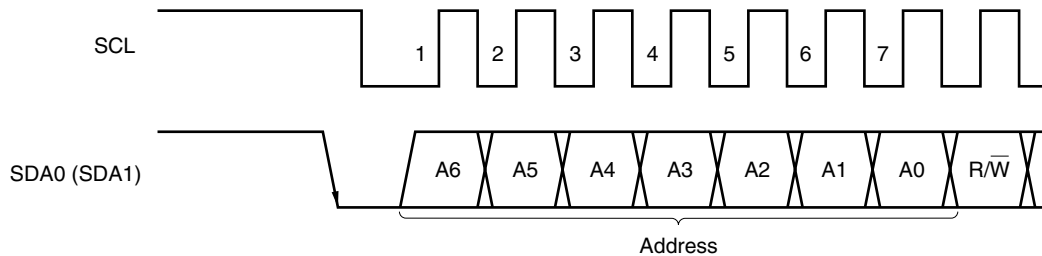
Figure 17-16. Address
