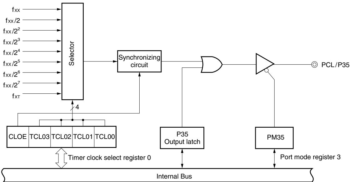
Figure 12-2. Clock Output Controller Block Diagram
