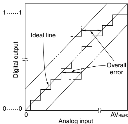
Figure 14-9. Overall Error
