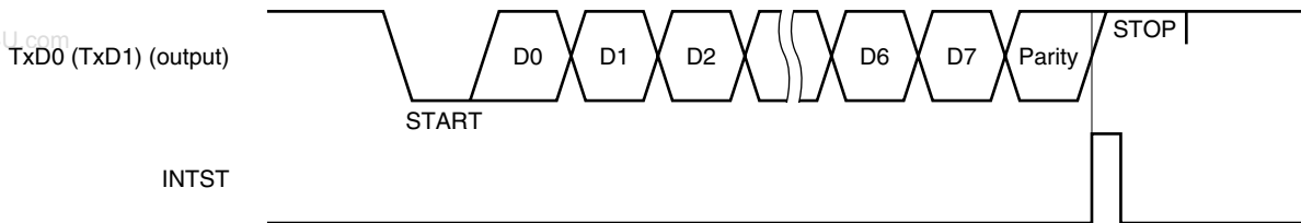
(a) Stop bit length: 1
