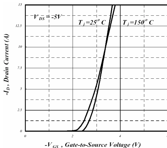
Fig 11. Transfer Characteristics
