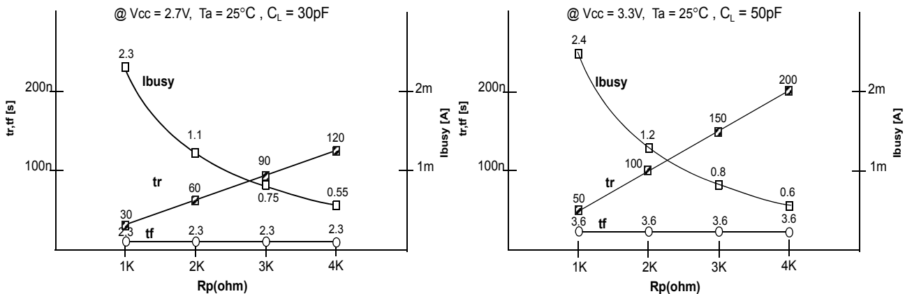
Figure 22. Rp vs tr ,tf & Rp vs i busy
