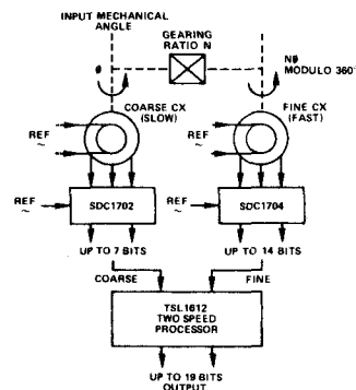
Diagram Showing Coarse/Fine Synchro Processor System
