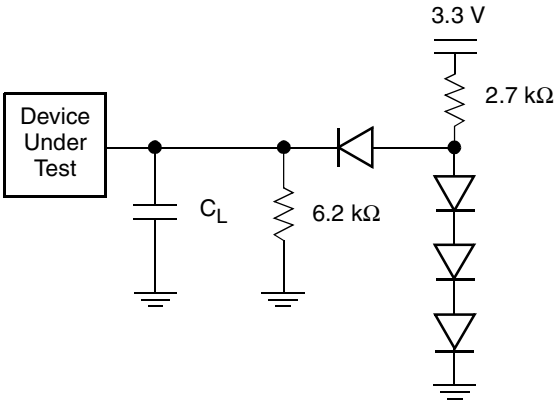
Figure 13. Test Setup
