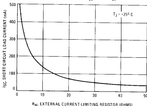
FIGURE 11 - I_{\text{SC}} versus R_{\text{SC}}
