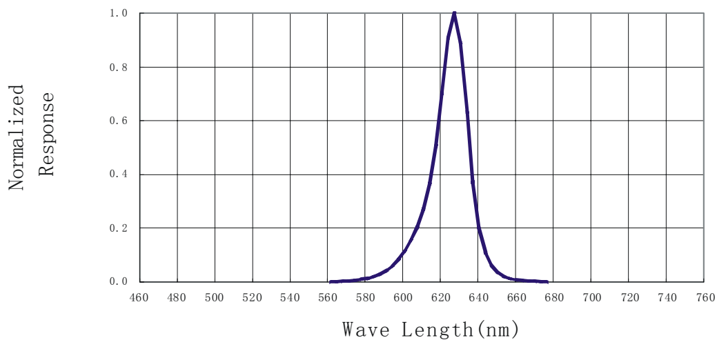
Spectral Radiance (Peak @ 632 nm)
