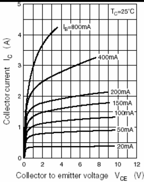
Fig.3 Static Characteristic
