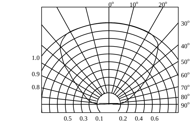
FIG.5 Radiation Characteristic I_{\text{rel}} = f(j)
