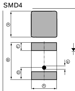
SMD4 C_b=0.24\text{pF}
