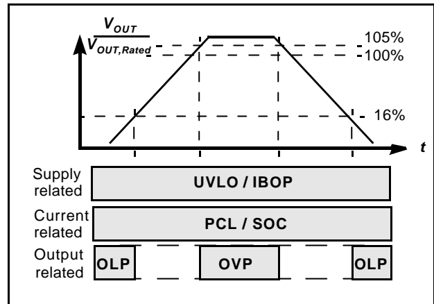
Figure 6 Protection Features
