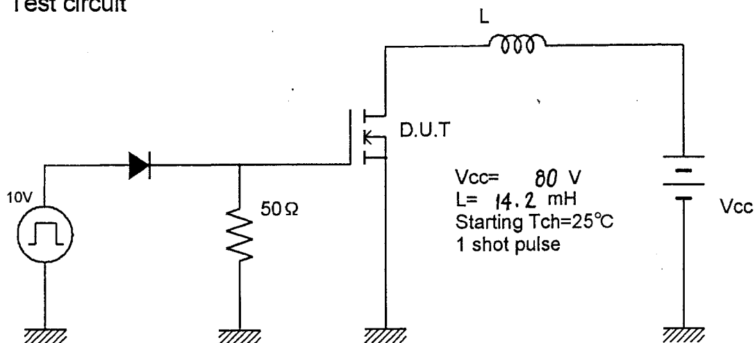
Fig.1 Test circuit
