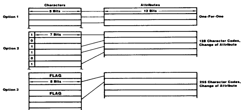
Figure 2. Attribute Fetch
