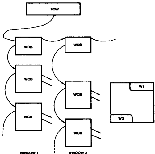
Figure 6. Window Data Structure
