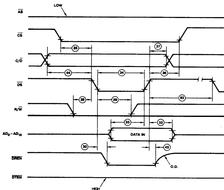
Am8052 Bus Slave Write Unlatched
