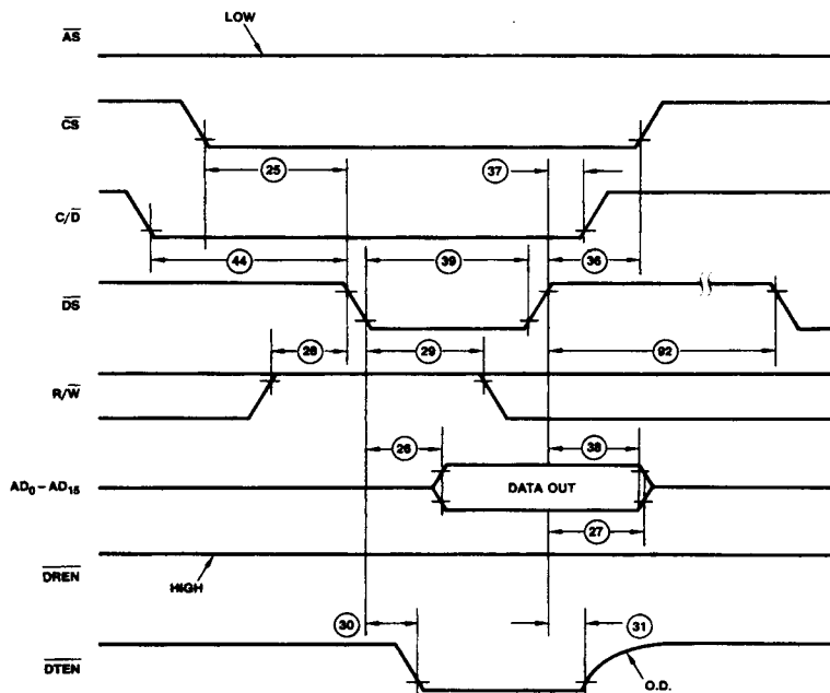
Am8052 Bus Slave Read Unlatched
