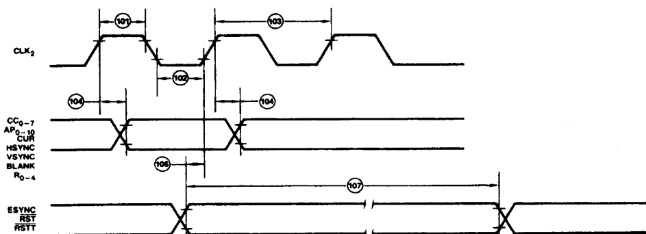
Am8052 Video Outputs and Synchronizing Input Timing
