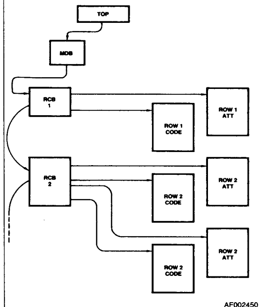
Figure 5. Background Data Structure
