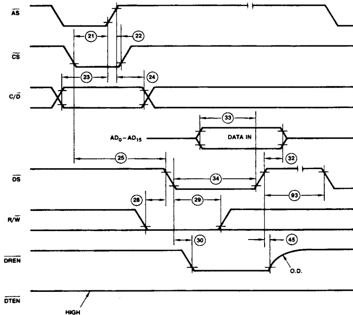
Am8052 Bus Slave Write Latched
