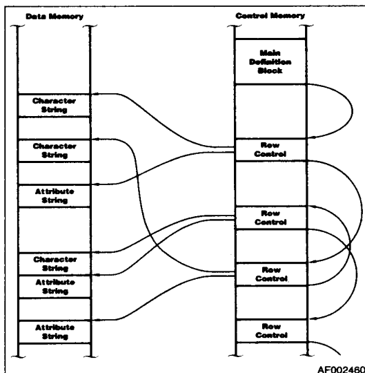
Figure 4. Am8052 Linked-List Structure
