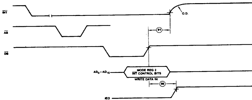
Am8052 Non-Vectored INT Timing
