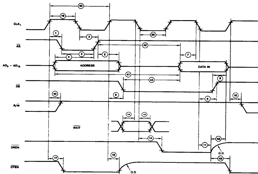
Am8052 Bus Master Read
