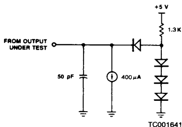
Standard Test Load
