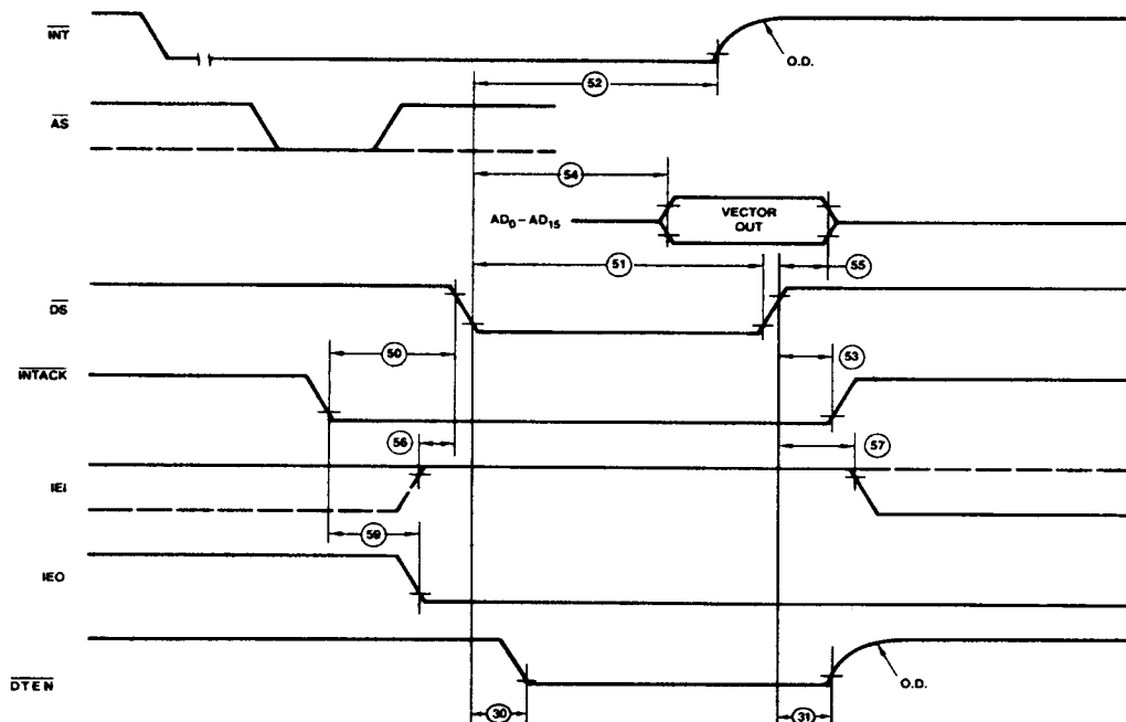
Am8052 Interrupt ACK Timing - Device Acknowledged
