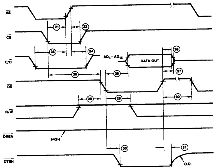
Am8052 Bus Slave Read Latched
