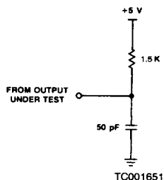
Open-Drain Test Load
