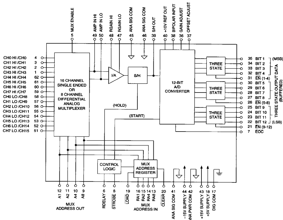
Figure 1. HDAS-16 and HDAS-8 Functional Block Diagram
