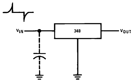
FIGURE 3. Transients
