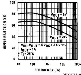
Ripple Rejection
