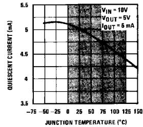
Quiescent Current
