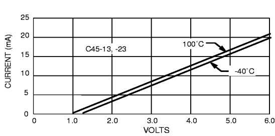
INPUT CURRENT VS CONTROL VOLTAGE FIGURE 1
