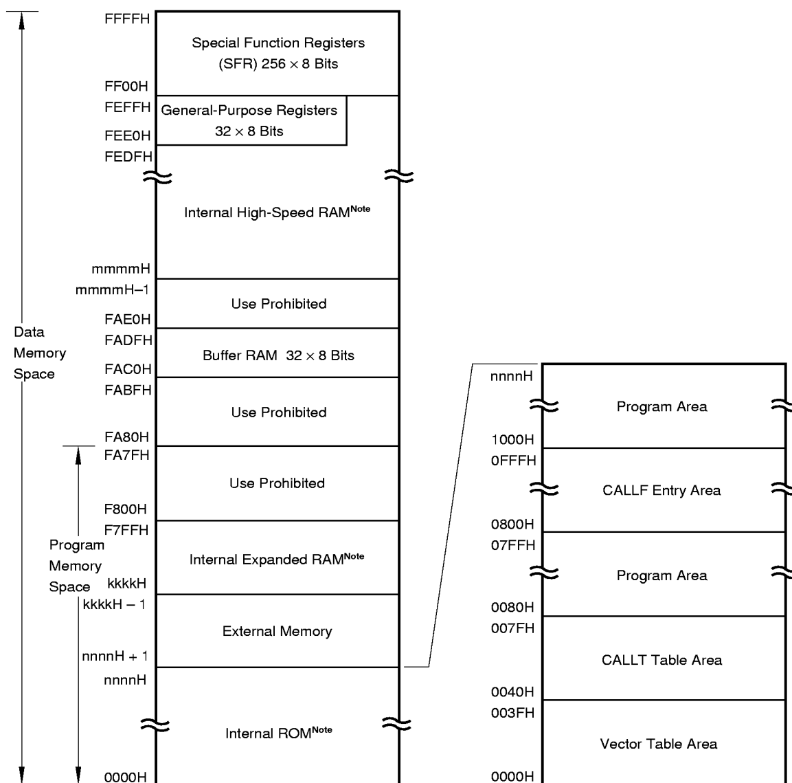
Figure 4-2. Memory Map ( \mu PD78015F, 78016F, 78018F)
