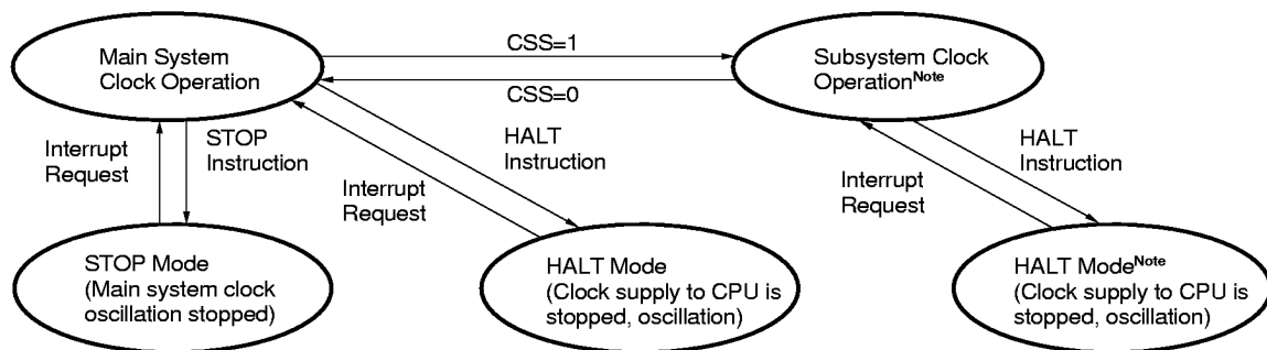
Figure 8-1. Standby Functions
