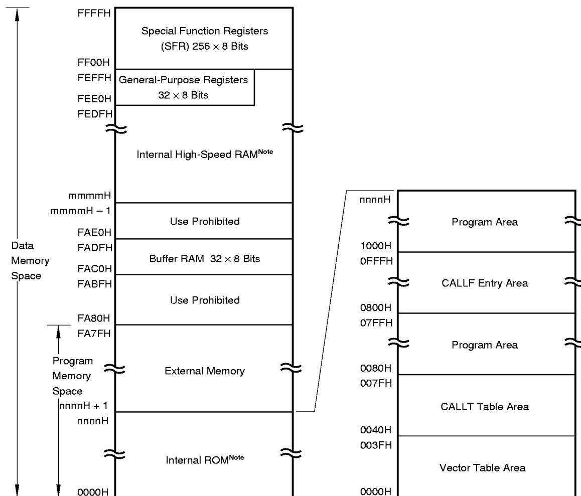
Figure 4-1. Memory Map (μPD78011F, 78012F, 78013F, 78014F)
