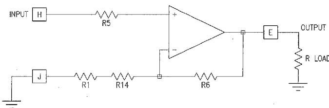
FIGURE 4. Non-inverting Amplifier Circuit
