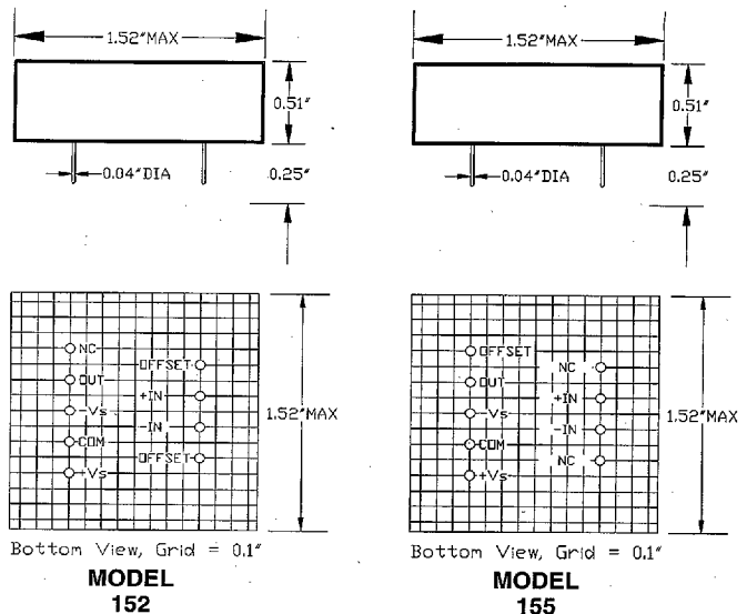
FIGURE 7. Outline Dimensions
