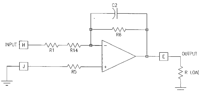
FIGURE 1. Inverting Amplifier
