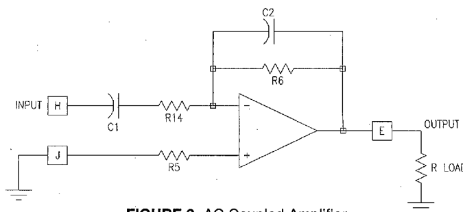
FIGURE 3. AC Coupled Amplifier
