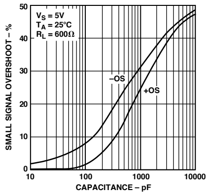
Figure 23. Small Signal Overshoot vs. Load Capacitance
