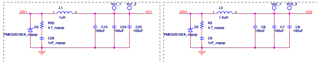
Figure 6. 34717 Typical Application
