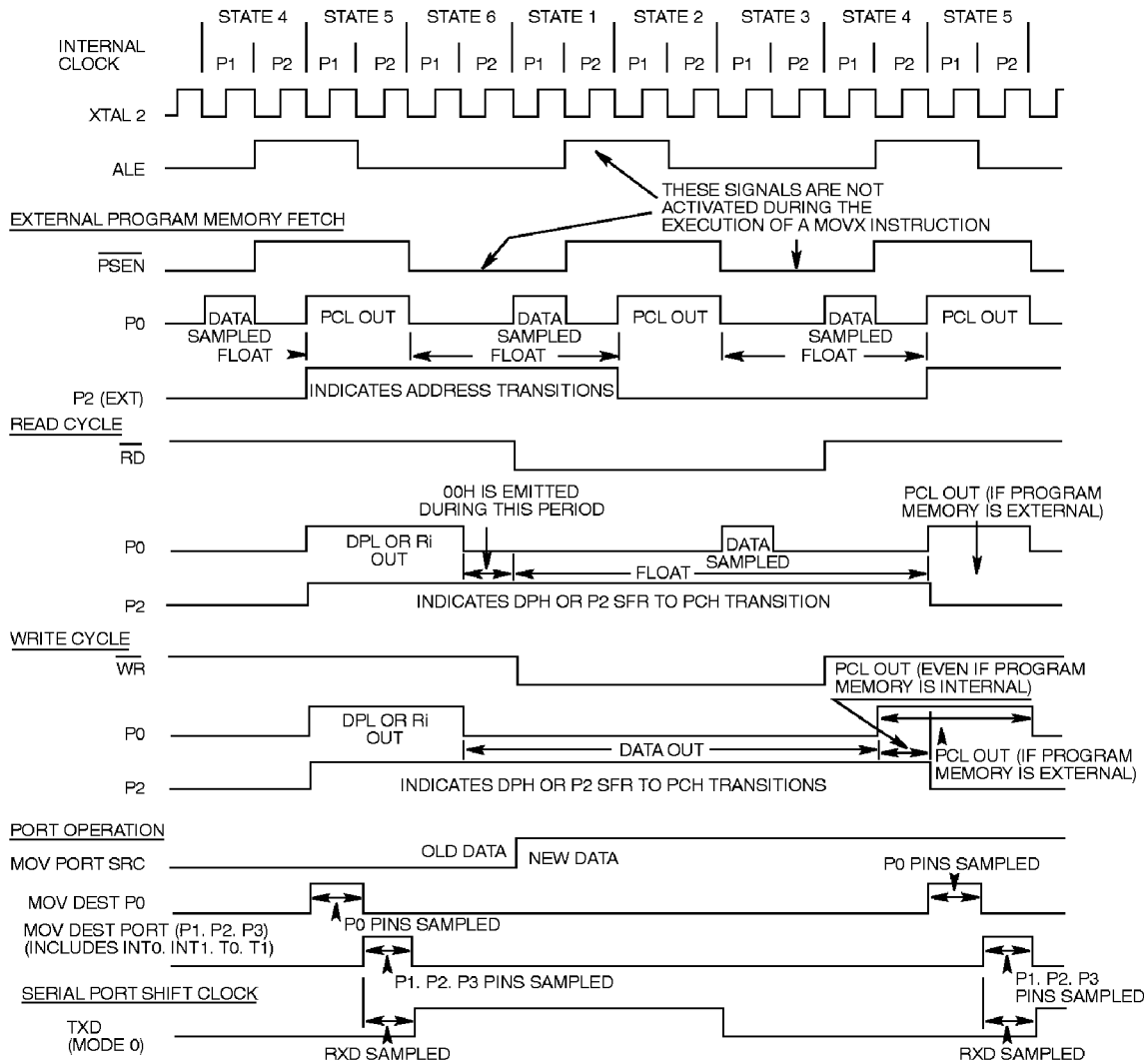
Figure 20. Clock Waveforms
