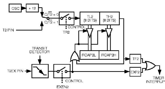
Figure 8. Timer in Auto-Reload Mode.
