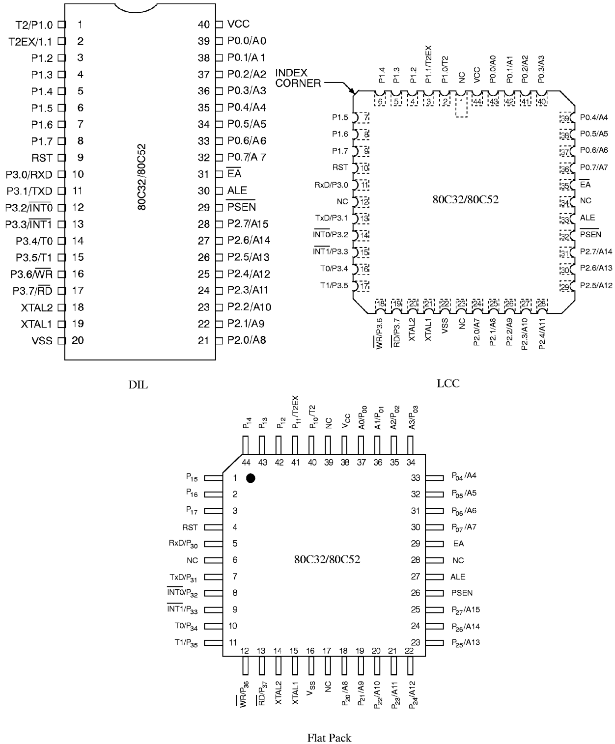
Figure 2. Pin Configuration
