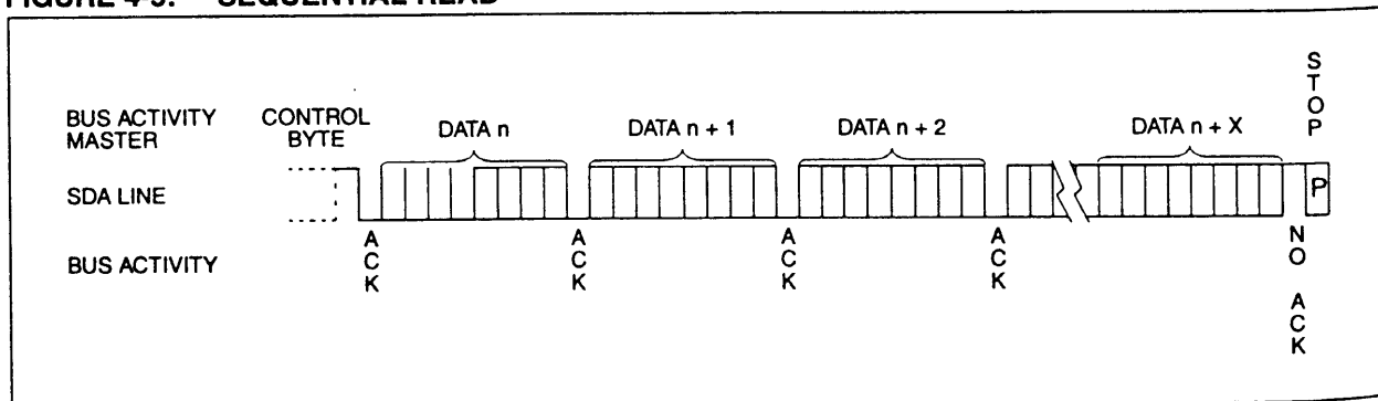
FIGURE 4-5: SEQUENTIAL READ
