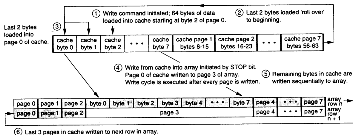
FIGURE 8-3: CACHE WRITE TO THE ARRAY STARTING AT A NON-PAGE BOUNDARY
