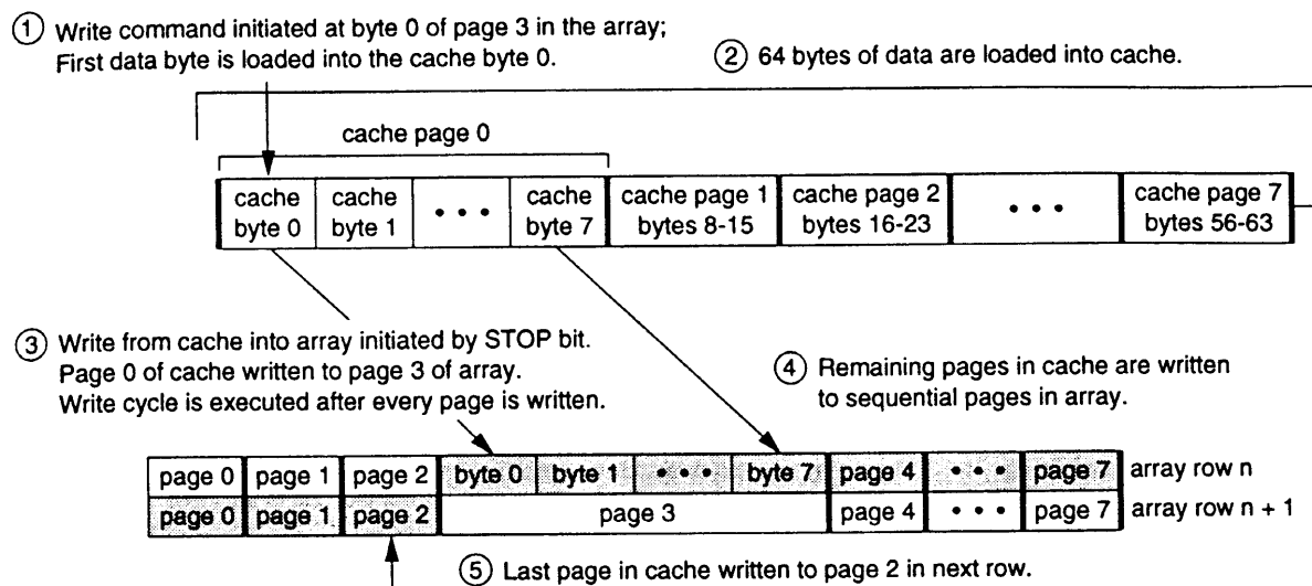
FIGURE 8-2: CACHE WRITE TO THE ARRAY STARTING AT A PAGE BOUNDARY
