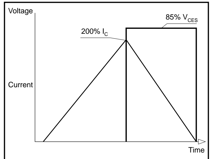
Fig. 13 Idealized waveforms
