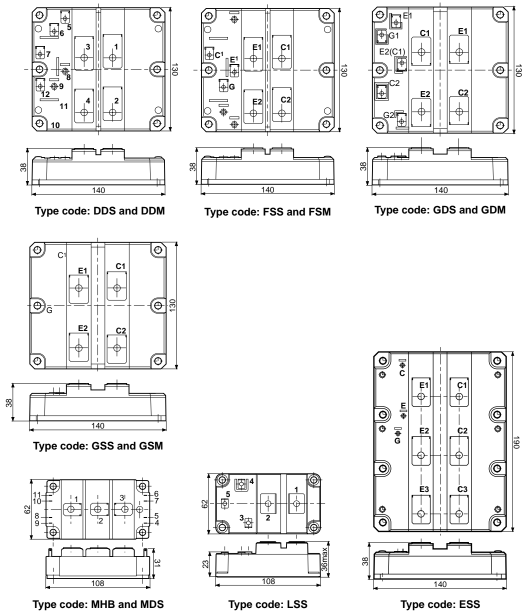
Fig.2 IGBT packages used by Dynex Semiconductor
