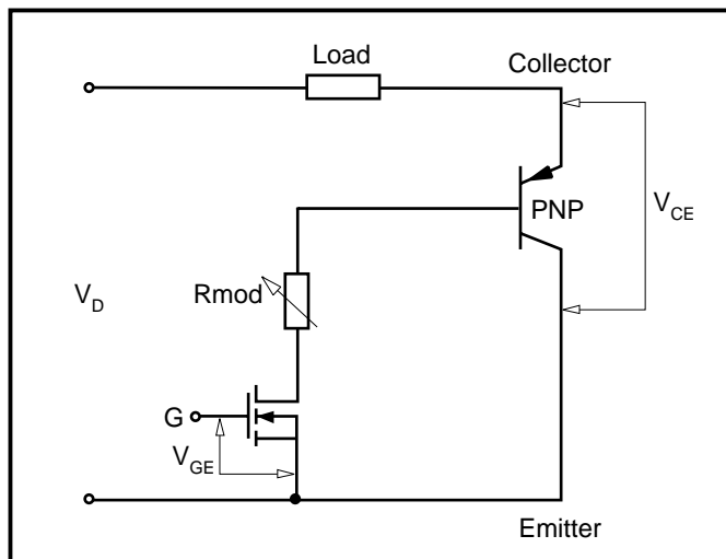
Fig. 1 IGBT equivalent circuit showing basic parameters
