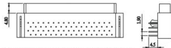
ALL PLASTIC TYPE FOR 68 POSITION FEMALE
