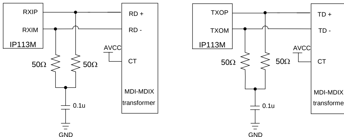
IP113M's application circuit (auto MDI-MDIX on)
