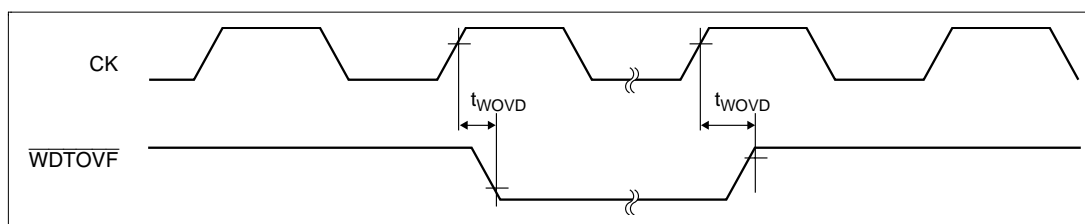
Figure 26.26 Watchdog Timer Timing
