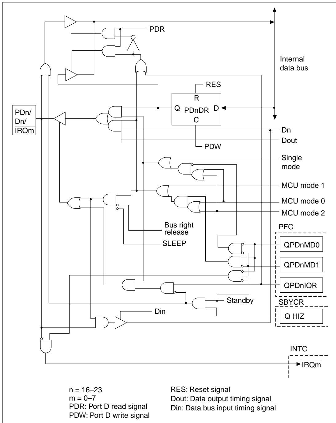
Figure B.26 PDn/Dn/IRQm Block Diagram (n = 16-23)
