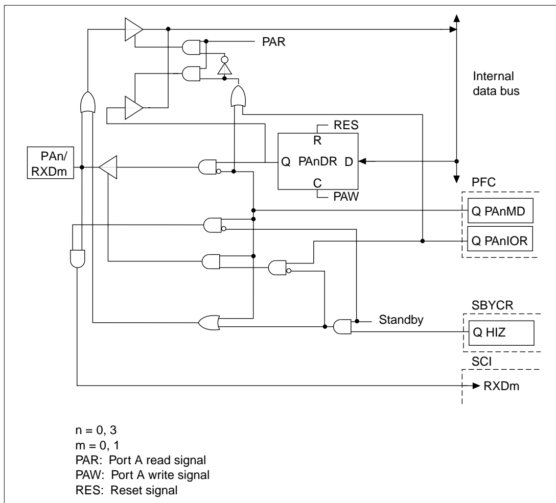
Figure B.1 PAn/RXDm Block Diagram
