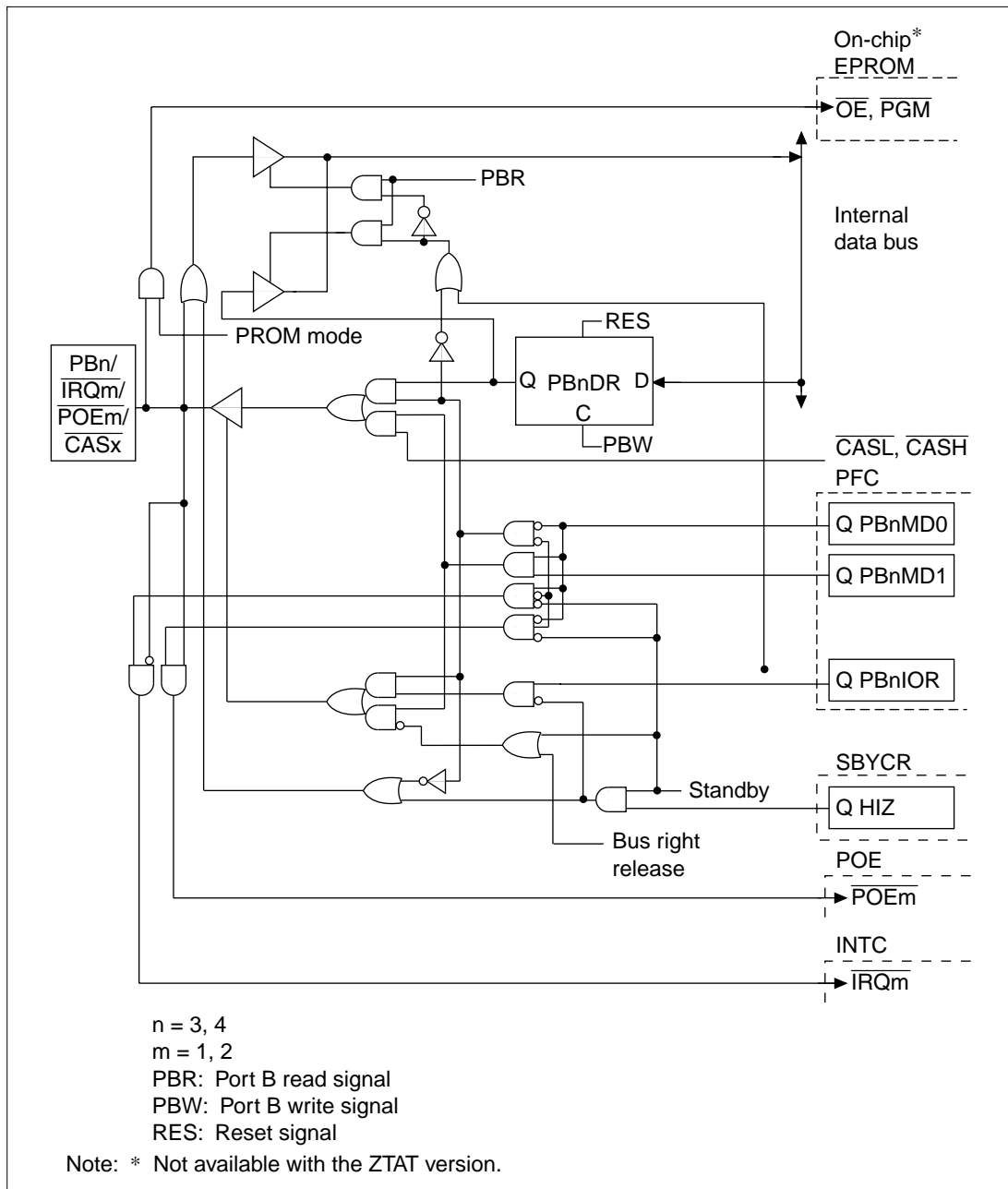
Figure B.18 \overline{\text{PBn}}/\overline{\text{IRQm}}/\overline{\text{POEm}}/\overline{\text{CASx}} Block Diagram
