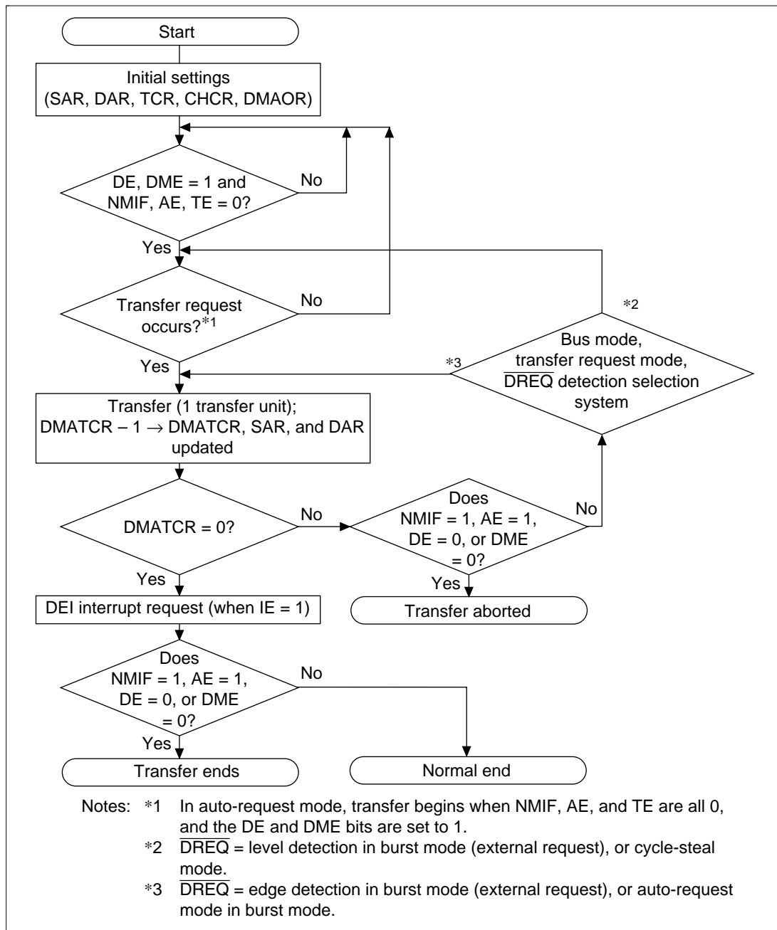
Figure 11.2 DMAC Transfer Flowchart
