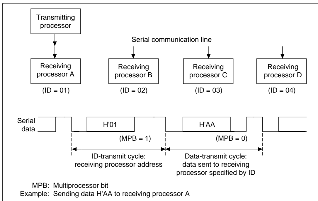
Figure 14.10 Communication among Processors Using Multiprocessor Format
