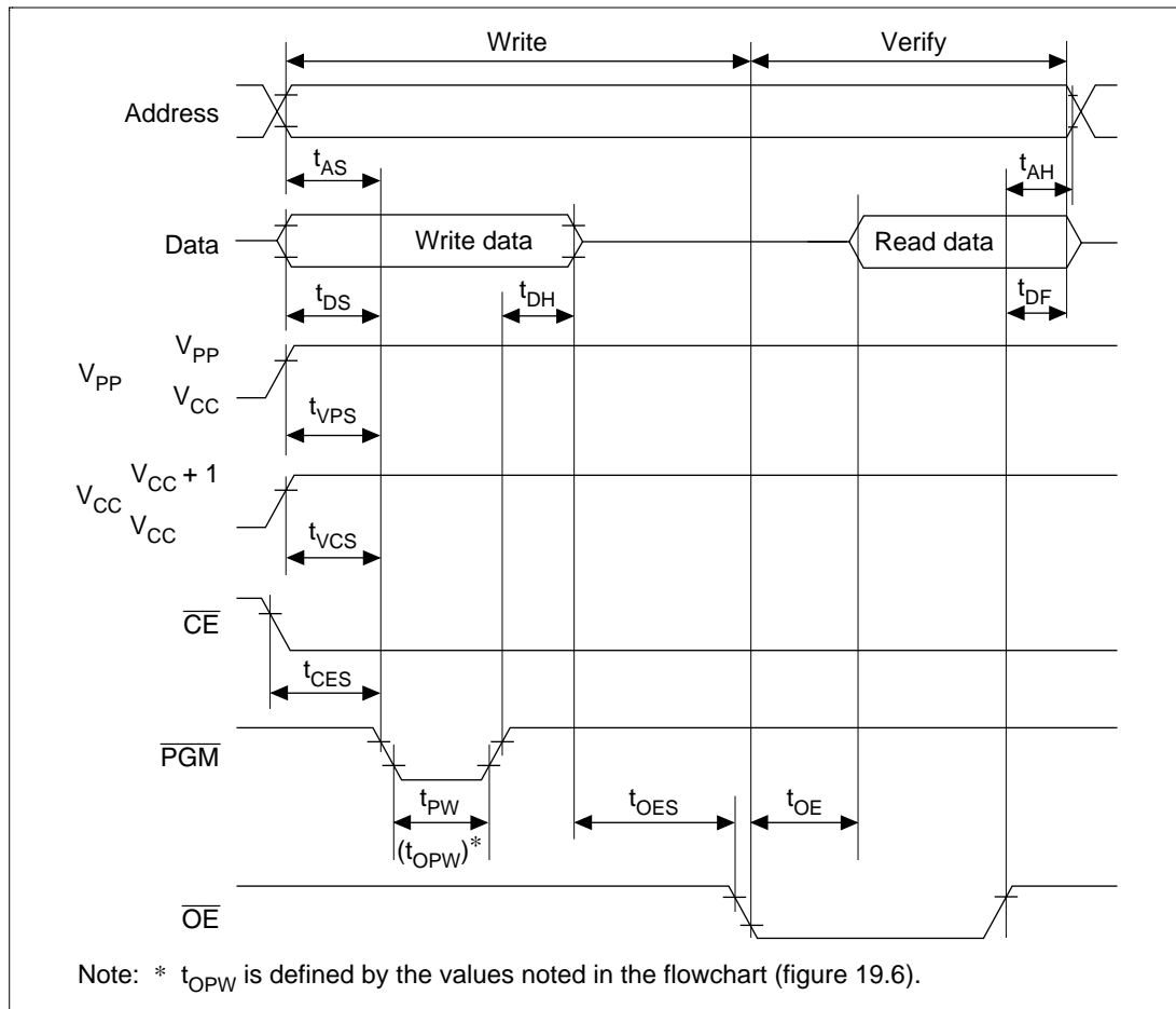
Figure 21.7 Write/Verify Timing
