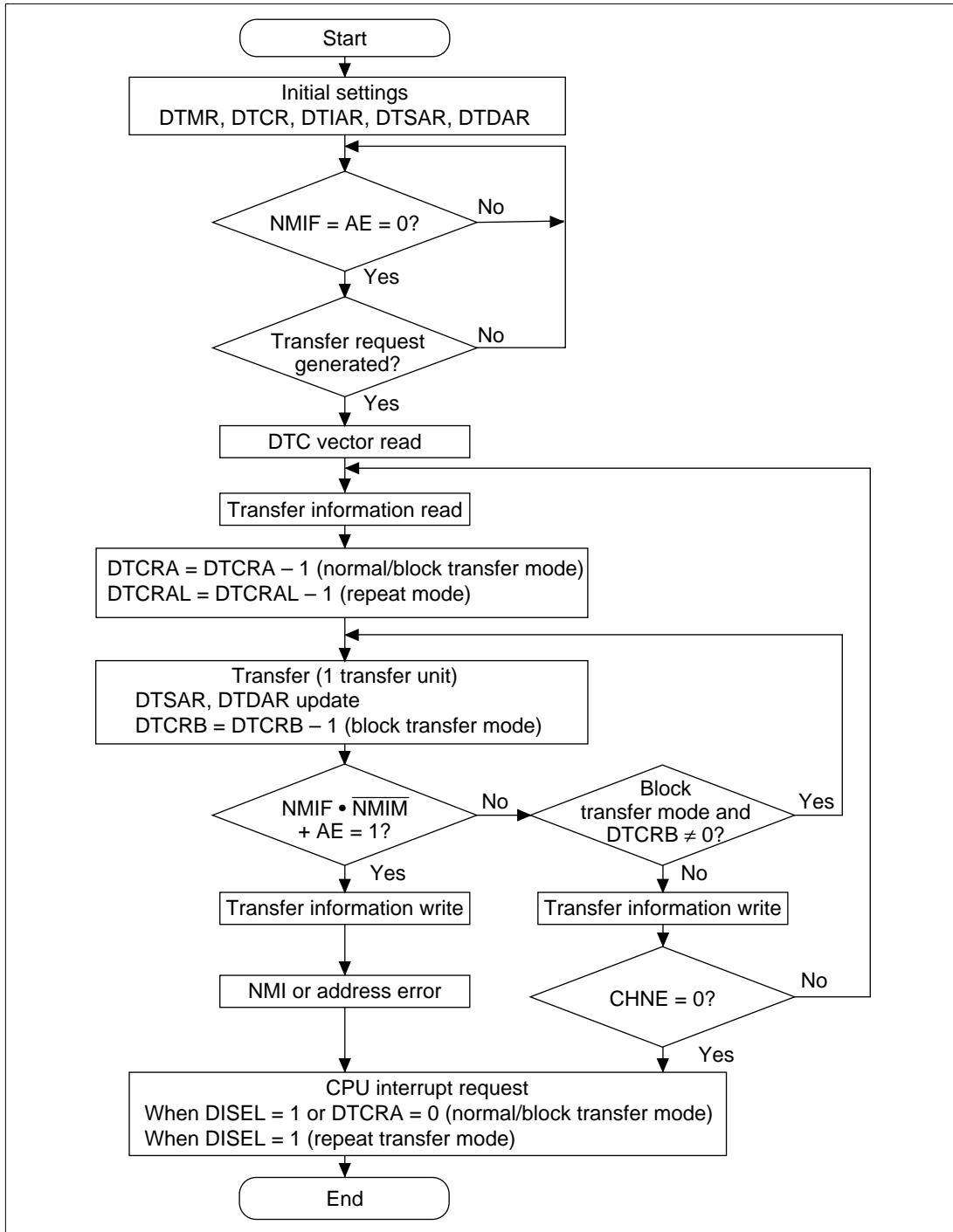
Figure 8.2 DTC Operation Flowchart
