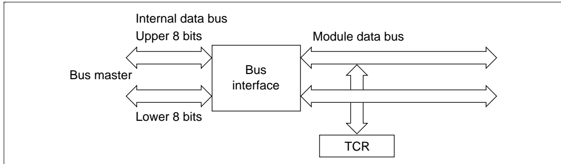
Figure 12.4 8-Bit Register Access Operation (Bus Master ↔ TCR (Upper 8 Bits))
