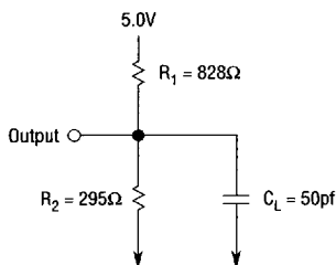
Load Circuit
