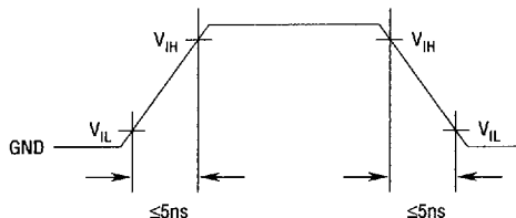
Input Waveforms
