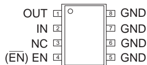
AAT3221 SC70JW-8 (Top View)
