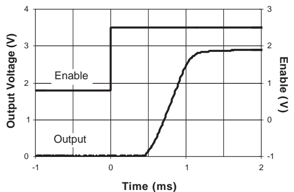
Turn-On with 100mA Load
