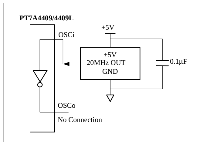
Figure 9. Clock Oscillator Connection
