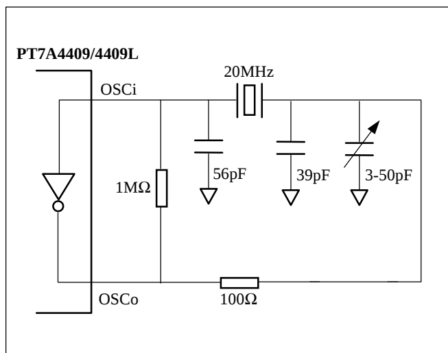
Figure 10. Crystal Oscillator Connection
