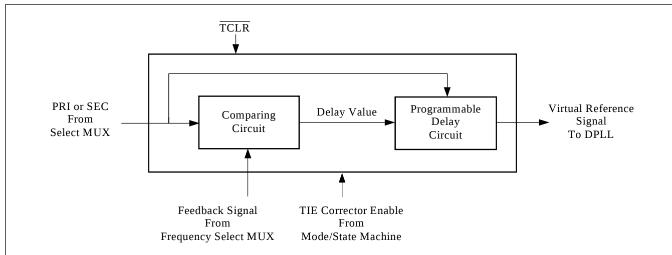
Figure 3. TIE Corrector
