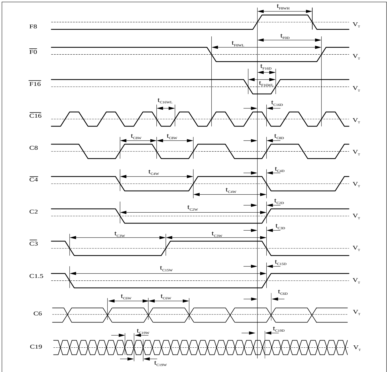
Figure 18. Output Timing
