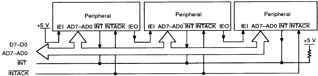
Figure 6. Z-Bus Interrupt Schedule
