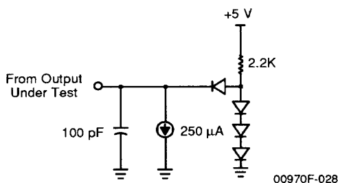
Standard Test Load
