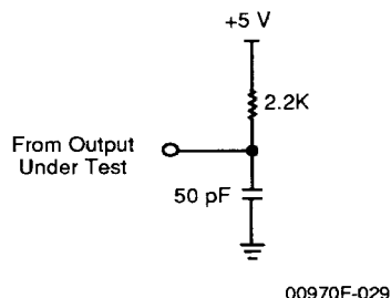
Open-Drain Test Load
