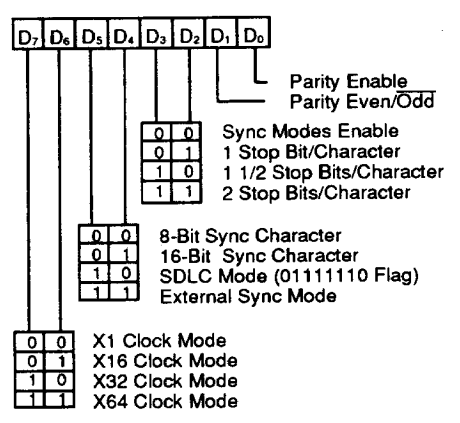
Figure 8. Write Register Bit Functions (Continued)
