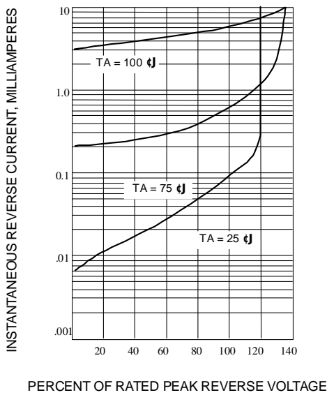
Fig. 3-TYPICAL REVERSE CHARACTERISTICS
