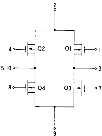
Equivalent circuit
