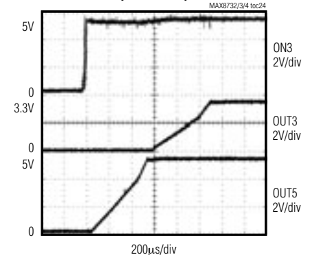
DELAYED START WAVEFORMS (ON3 = REF)
