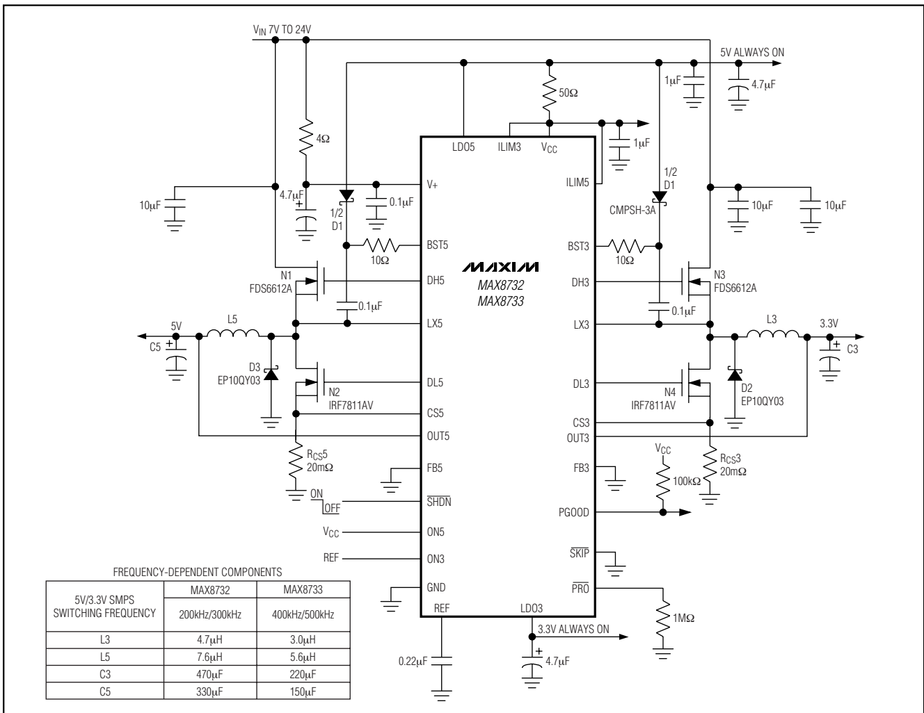
Figure 1. MAX8732/MAX8733 Typical Application Circuit
