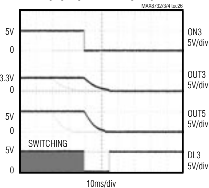
SHUTDOWN WAVEFORMS
