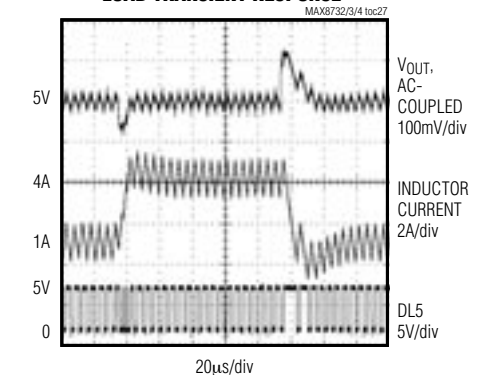
MAX8732/MAX8734 (TON = VCC) 5V PWM-MODE LOAD TRANSIENT RESPONSE
