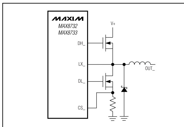
Figure 8. Current Sensing Using Sense Resistor (MAX8732/MAX8733)
