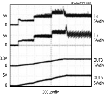
SOFT-START WAVEFORMS
