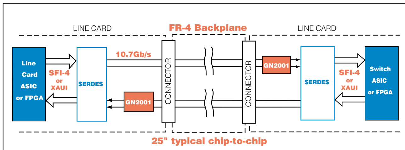
TYPICAL APPLICATION
