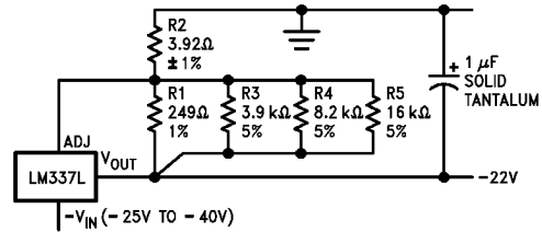
Regulator with Trimmable Output Voltage
