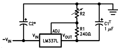
1.2V-25V Adjustable Regulator
