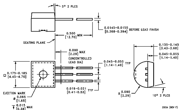
TO-92 Plastic Package (Z) Order Number LM337LZ NS Package Number Z03A
