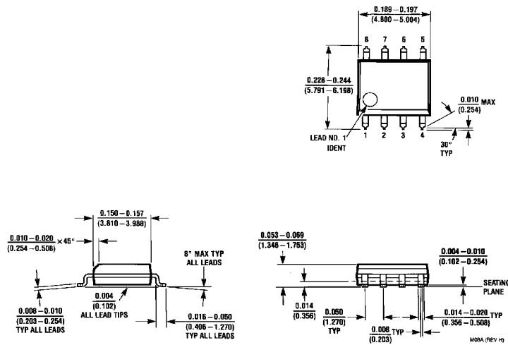
SO-8 Plastic Package (M) Order Number LM337LM NS Package Number M08A
