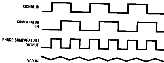
FIGURE 4. Typical Phase Comparator I. Waveforms
