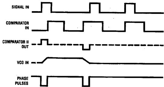
FIGURE 7. Typical Phase Comparator II Output Waveforms
