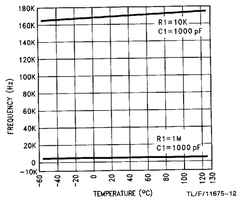
VHC4046 VCO out vs Temperature \text{V}_{\text{CC}} = 6\text{V}
