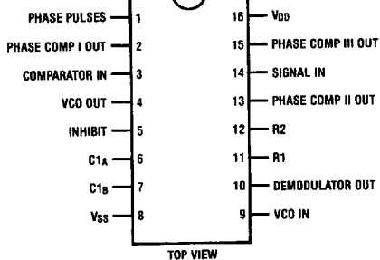
Pin Assignment for SOIC and PDIP
