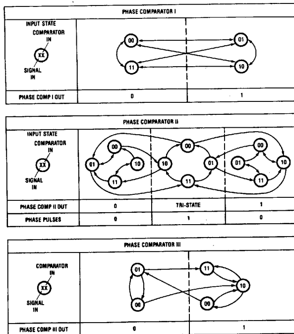
FIGURE 5. PLL State Tables
