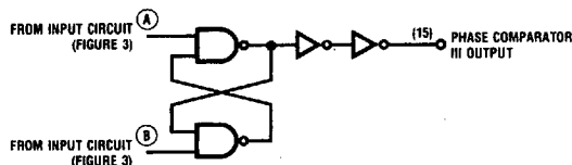
FIGURE 8. Phase Comparator III Logic Diagram
