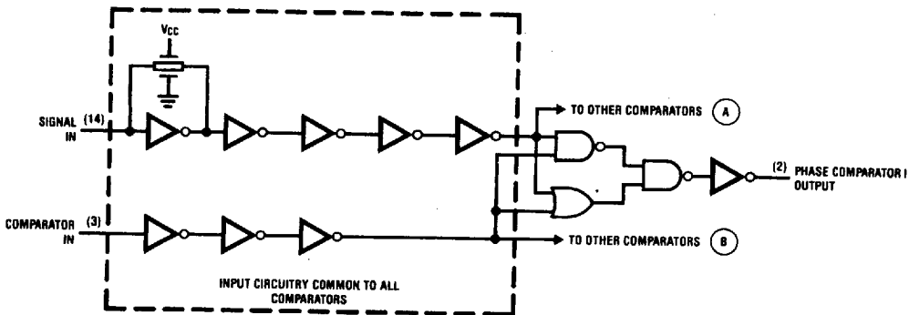
FIGURE 3. Logic Diagram for Phase Comparator I and the Common Input Circuit for All Three Comparators
