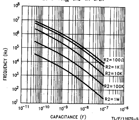
Typical Offset Frequency vs R2, C1 V_{CC} = 4.5V
