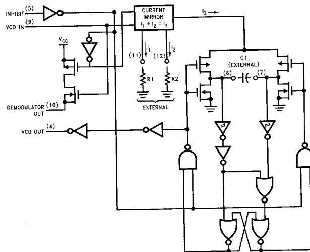
FIGURE 2. Logic Diagram for VCO
