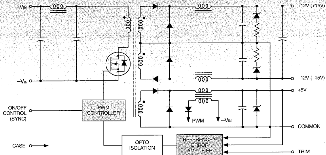
Figure 1. Simplified Schematic
