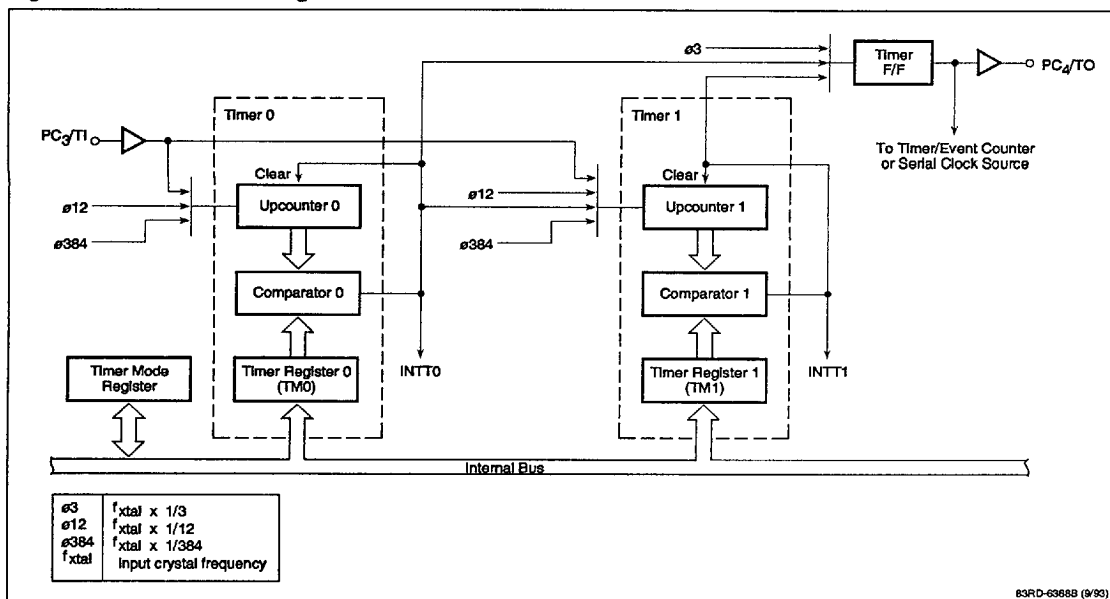
Figure 2. Timer Block Diagram
