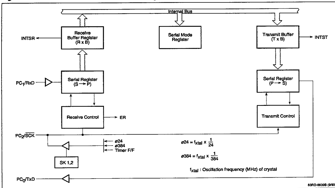
Figure 6. Universal Serial Interface Block Diagram
