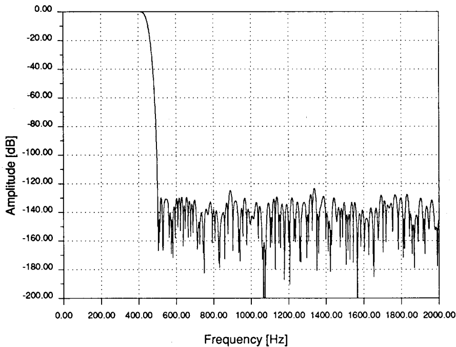
Figure A1.2. Second Stage Off-chip Filter – Magnitude Plot
