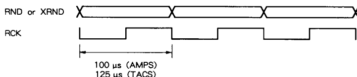
Fig. 2. Timing of RCK with RND or XRND
