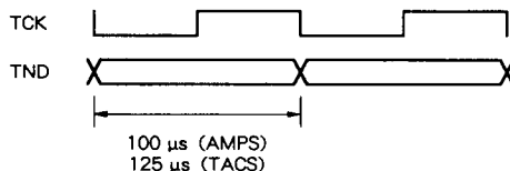
Fig. 3. Timing of TCK and TND
