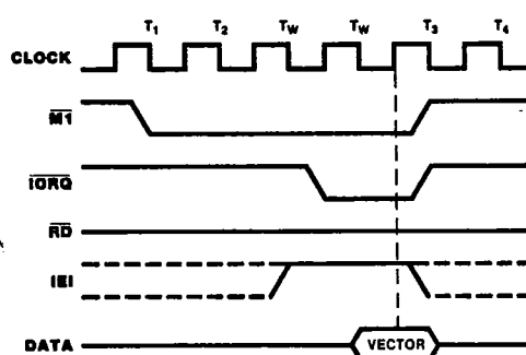
Figure 3. Interrupt Acknowledge Cycle
