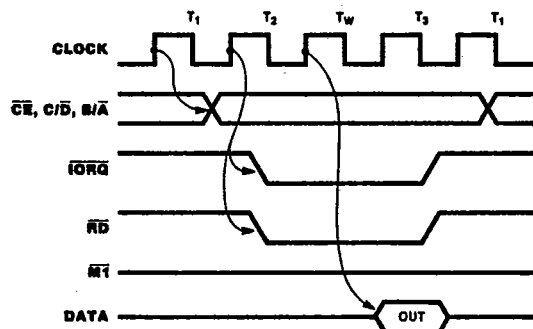
Figure 1. Read Cycle
