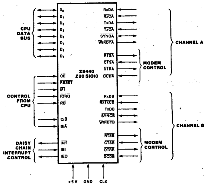
Figure 9. Pin Functions
