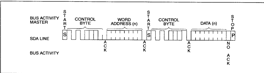
FIGURE 9-2: RANDOM READ
