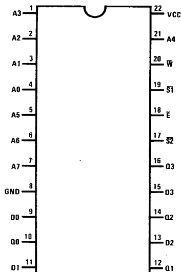
Dual-In-Line Package
