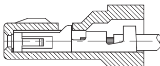
TERMINAL ASSEMBLY DRAWING
